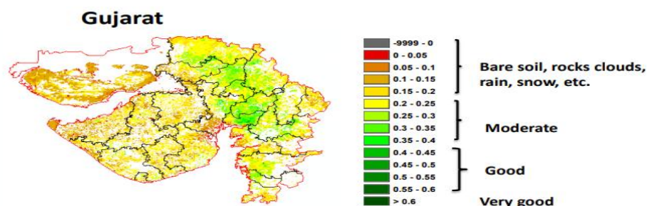
NOAA/VIIIRS/BLENDED NDVI Composite ending on Week no 12 (19.03.2021 to 25.03.2021) over Agricultural region
