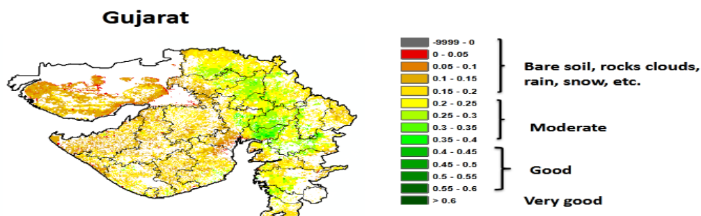
NOAA/VIIRS/BLENDED NDVI Composite ending on Week no 13 (26.03.2022 to 01.04.2022) over Agricultural region
