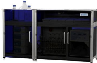
2D HPLC
